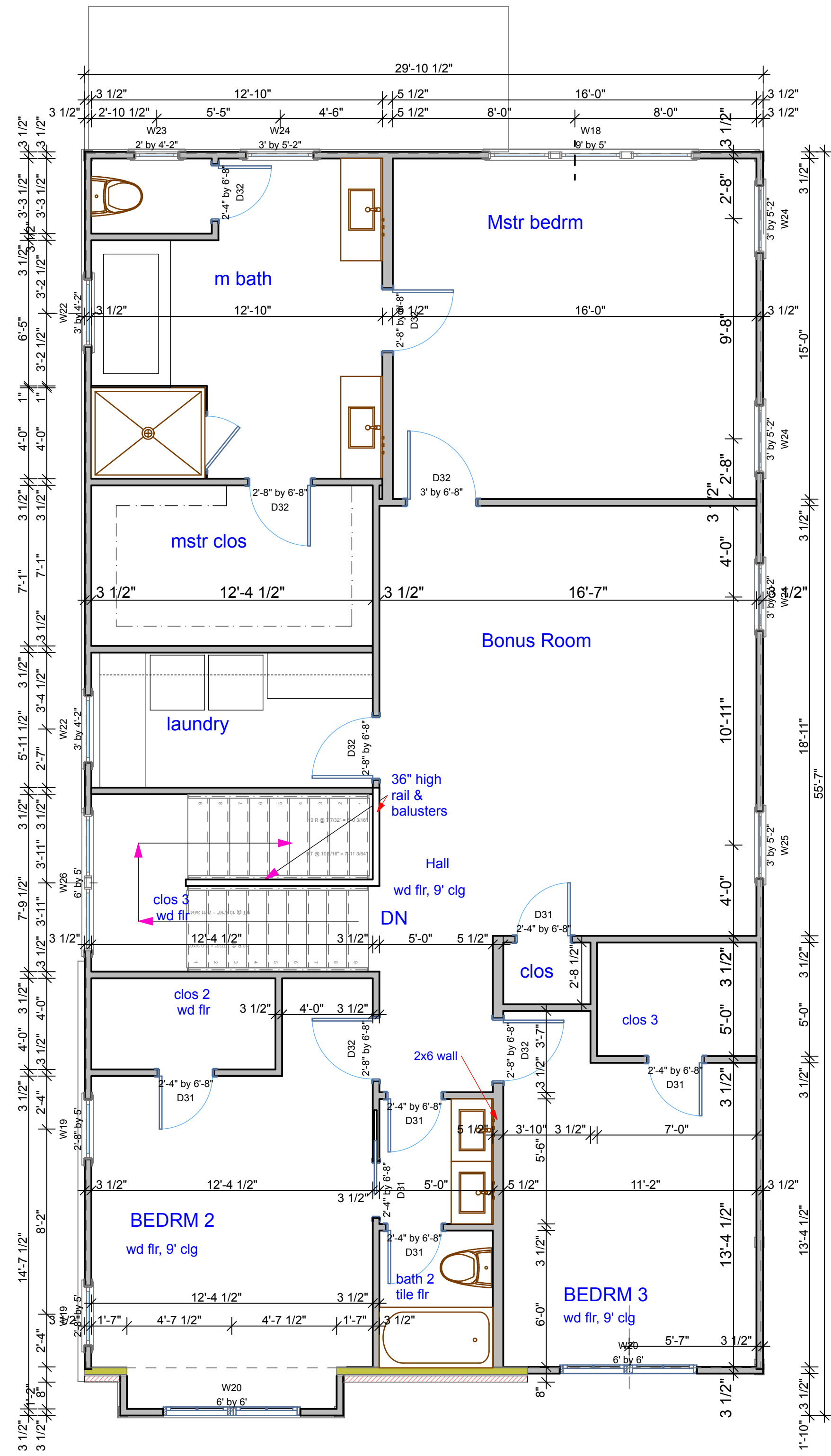
1 2ND FLR PLAN SCALE: 1/4" = 1'-0"
