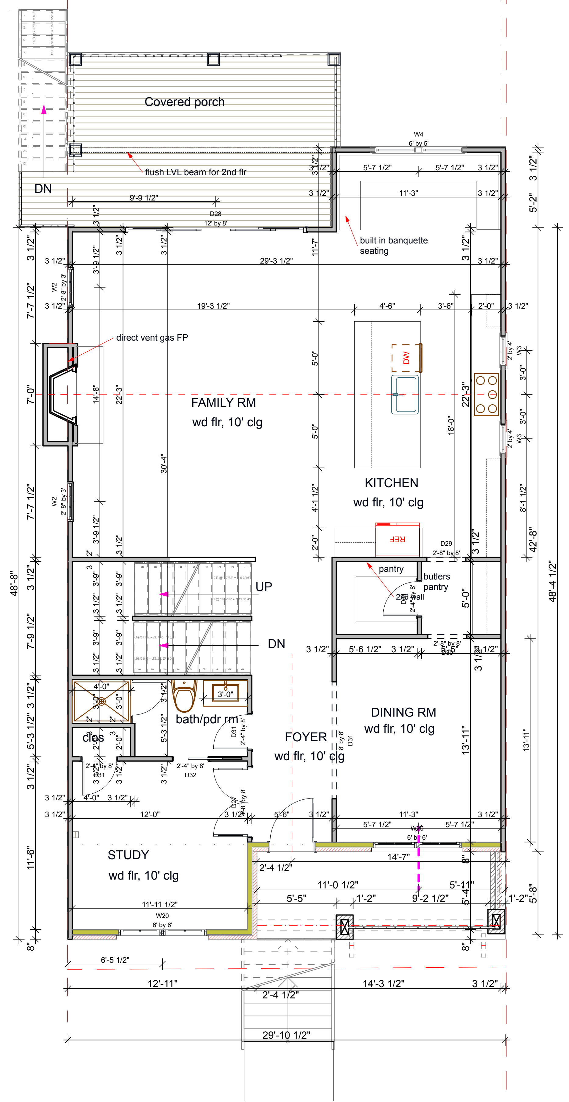
2 1ST FLR PLAN SCALE: 1/4" = 1'-0"
