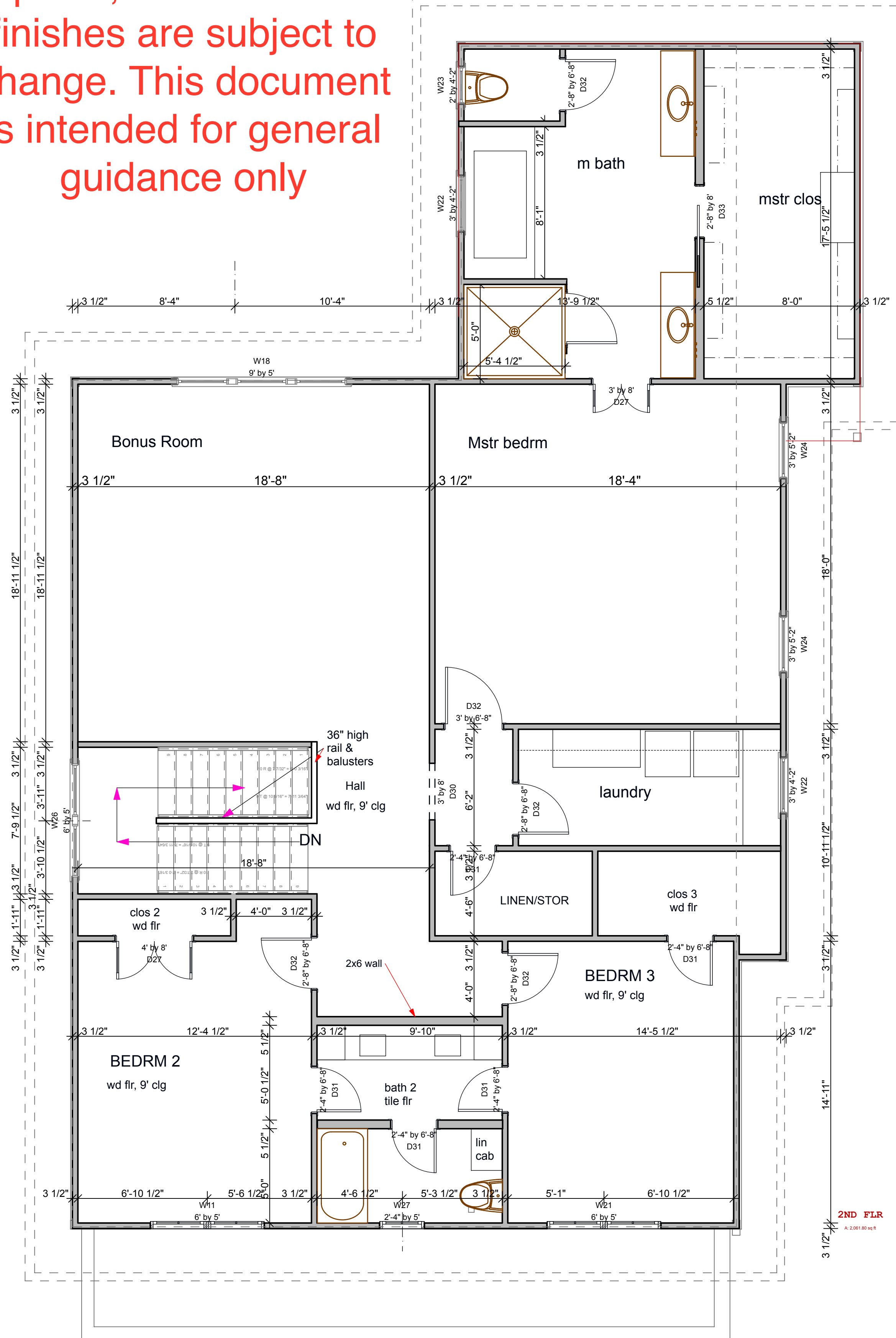
3 2ND FLR PLAN (2) SCALE: 1/4" = 1'-0"
