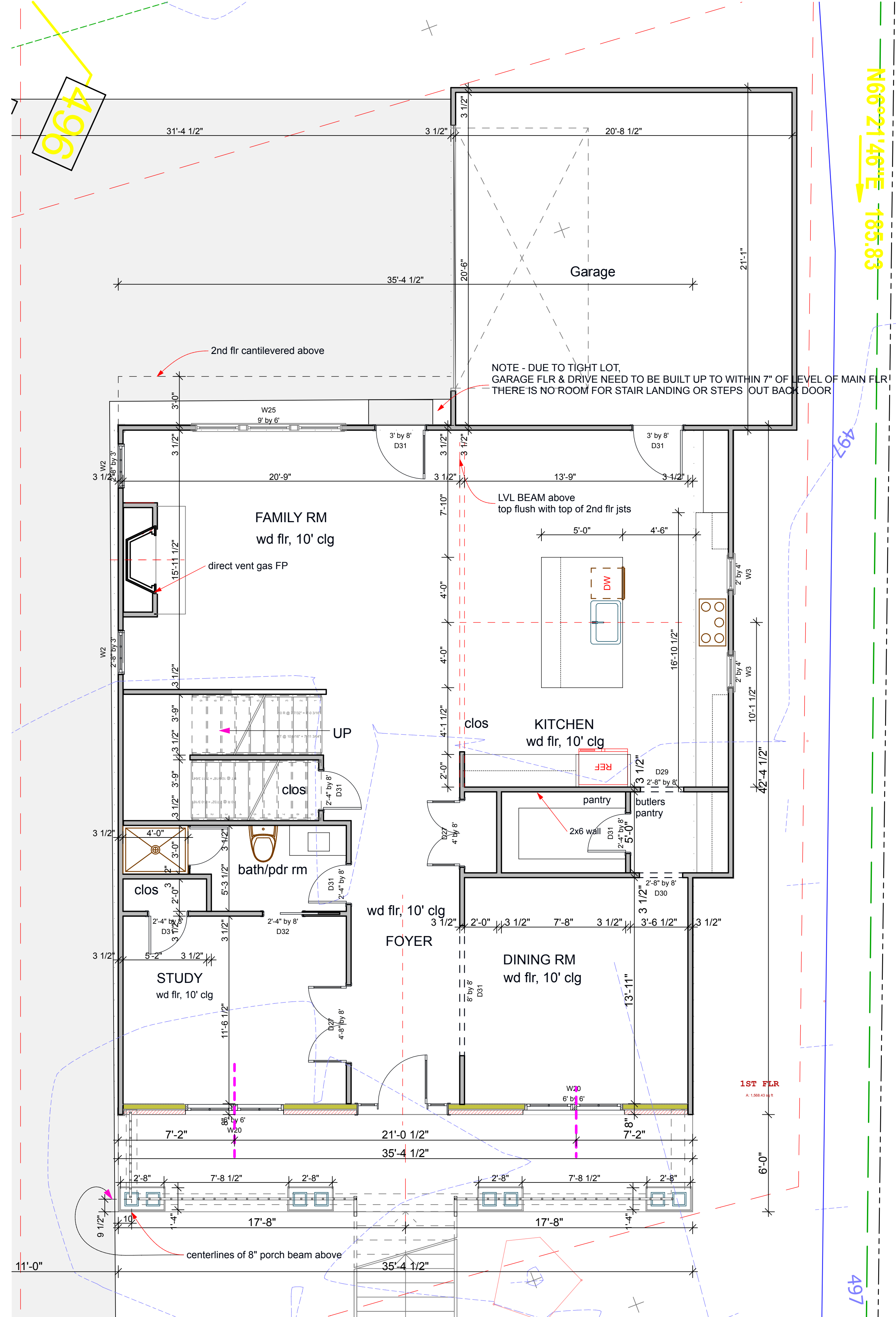
2 1ST FLR PLAN (3) SCALE: 1/4" = 1'-0"
